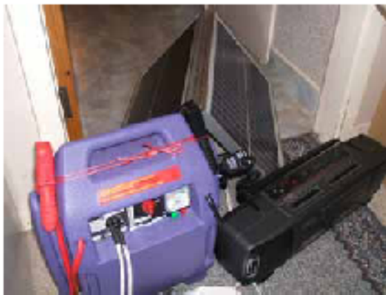
Justin's design: jump-start pack, and solar panel running a tape recorder as sent to Vanuatu
